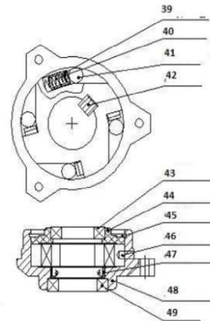
Clutch Assembly
